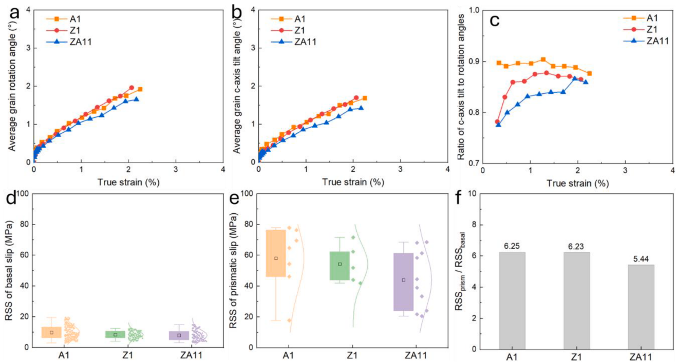
Fig. 5. (a) Average grain rotation angle and (b) c-axis tilt angle as functions of true strain of A1, Z1, and ZA11 alloys, (c) ratio of c-axis tilt to rotation angle of the three alloys, (d, e) resolved shear stresses (RSS) for basal and prismatic slips, and (f) ratios of RSS_{prism}/RSS_{basal} of the three alloys.
